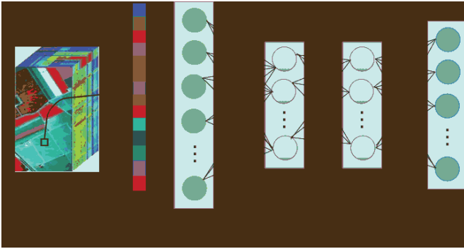
Fig. 11: RNN architecture
