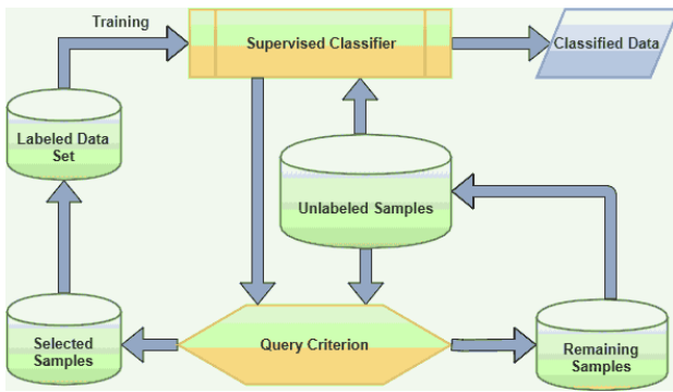
Fig. 14: A general overview of Active Learning
