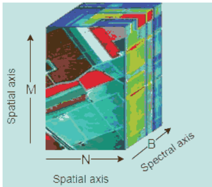
Fig. 4: Hyperspectral Cube
