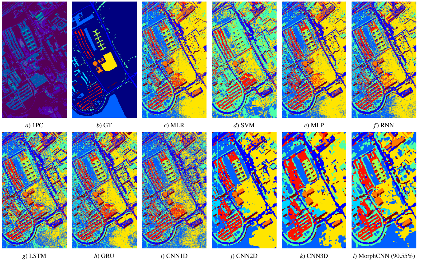
Fig. 20: Classification Maps obtained by MLR [321], SVM [322], MLP [69], RNN [70], LSTM [323], GRU [324], CNN-1D [218], CNN-2D [325], CNN-3D [326] and MorphCNN [196] on the disjoint train-test dataset for the UP scene.
